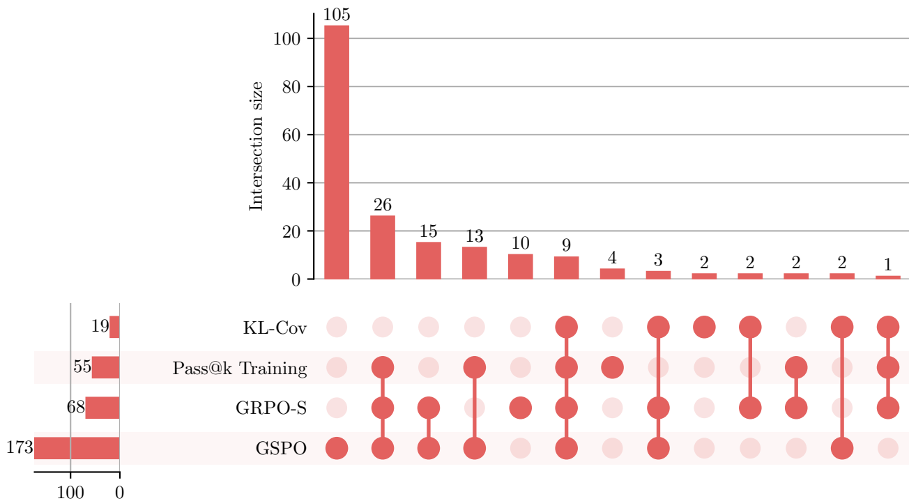
Shrinkage Intersections (pass@256 Base=1, RL=0), Model: EuroLLM-9B-Instruct
